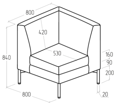
EV-GM-Y.01 800x800x840
