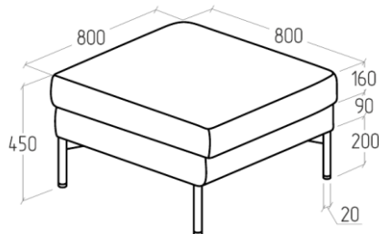
EV-GM-BY.01 800x800x450
