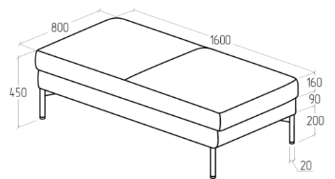
EV-GM-BY.02 1600x800x450
