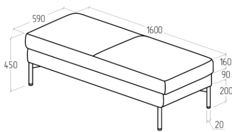
EV-GM-B.02 1600x590x450
