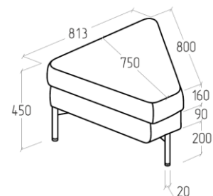
EV-GM-PFY 750x800x450
