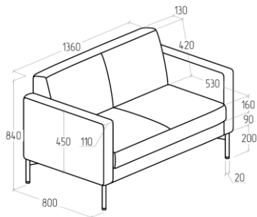
EV-GM-P.02 1360x800x840
