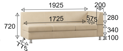
EV-MN-1P.03 (R/L) 1925x775x720
