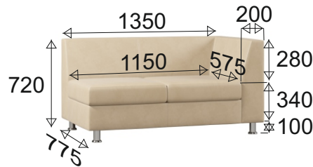
EV-MN-1P.02 (R/L) 1350x775x720
